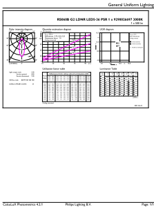
Downlight RS060B G2 LDNR 830 PSR WH-GUL
