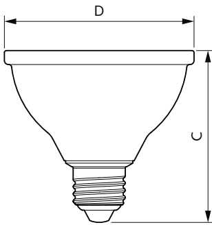
MAS LEDspot CLA D 9.5-75W 827 PAR30S 25D
