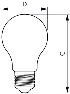
LEDbulb ND 10-75W A60 E27 827 6CT
