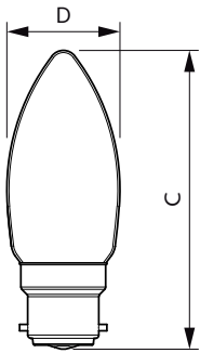
CorePro LEDCandleND 2-25W B35 B22 827CLG
