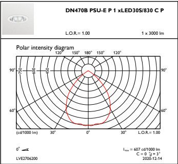
OFPC1_DN470BPSU-EP1xLED30S830CP
