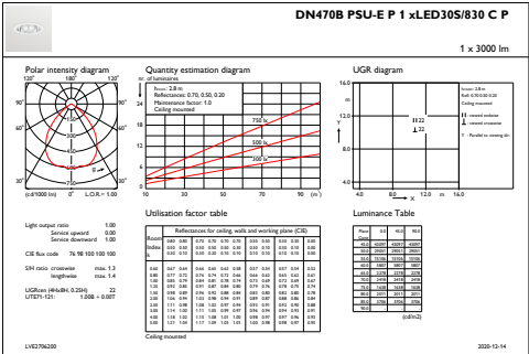
IFGU1_DN470BPSU-EP1xLED30S830CP
