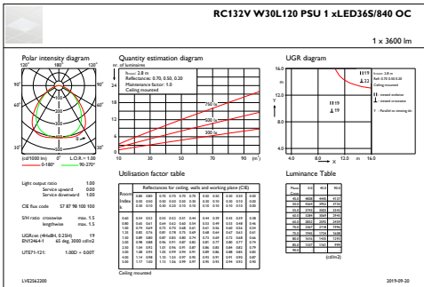
IFGU1_RC132VW30L120PSU1xLED36S840OC
