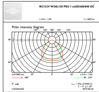
OFPC1_RC132VW30L120PSU1xLED36S840OC
