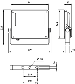
BVP125 LED80-4S/730 PSU S ALU C1KC3
