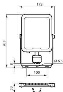
BVP164 LED55/830 PSU 50W SWB MDU CE
