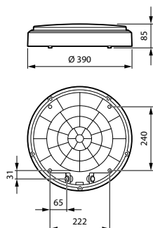
WL140V LED20S/830 PSU WH
