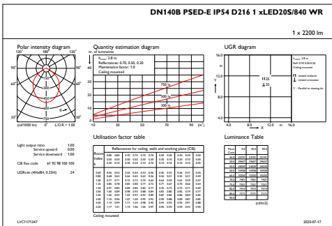
IFGU1_DN140BPSED-EIP54D2161xLED20S840WR
