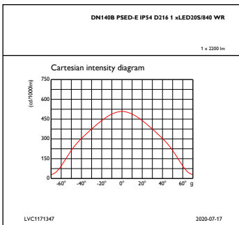
IFCC1_DN140BPSED-EIP54D2161xLED20S840WR
