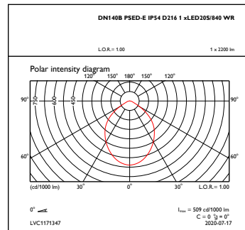
OFPC1_DN140BPSED-EIP54D2161xLED20S840WR
