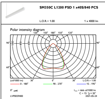
OFPC1_SM350CL1200PSD1x40S840PCS
