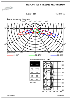
OFPL1_BGP291T251xLED20-4S740DM50
