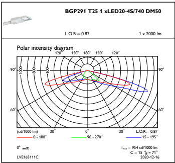
OFPC1_BGP291T251xLED20-4S740DM50
