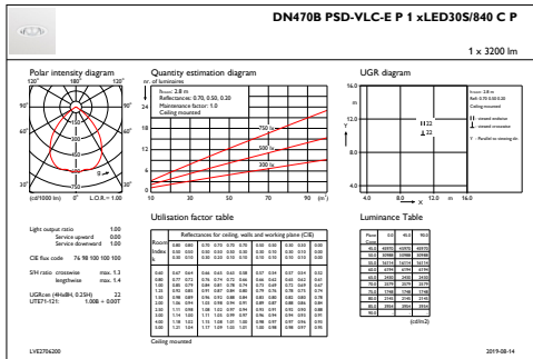
IFGU1_DN470BPSD-VLC-EP1xLED30S840CP
