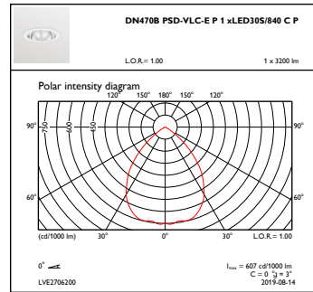
OFPC1_DN470BPSD-VLC-EP1xLED30S840CP
