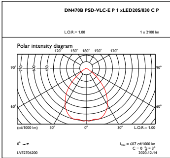
OFPC1_DN470BPSD-VLC-EP1xLED20S830CP
