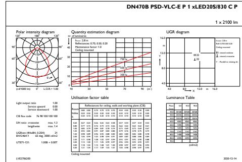
IFGU1_DN470BPSD-VLC-EP1xLED20S830CP
