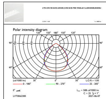
OFPC1_RC461BPSDW60L601xLED28SBU8400C
