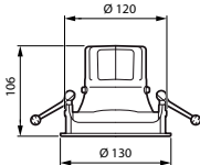
RS771B 49S/830 PSU-E HWB WH
