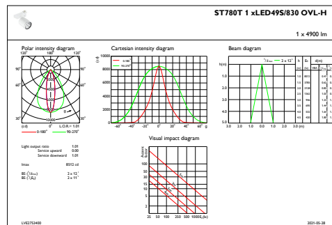
IFAS1_ST780T1xLED49S830OVL-H
