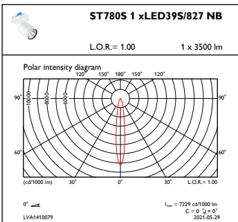
OFPC1_ST780S1xLED39S827NB
