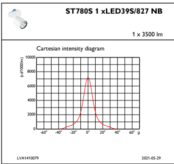
IFCC1_ST780S1xLED39S827NB
