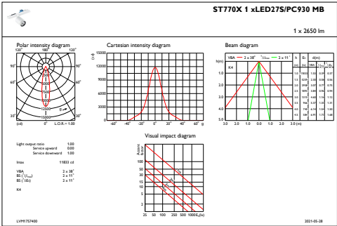
IFAS1_ST770X1xLED27SPC930MB
