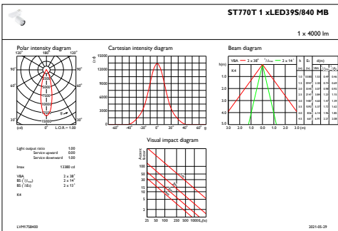
IFAS1_ST770T1xLED39S840MB
