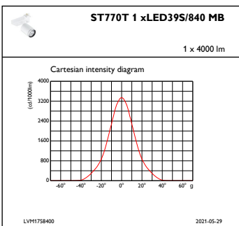
IFCC1_ST770T1xLED39S840MB
