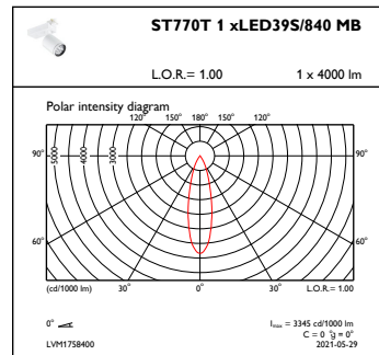
OFPC1_ST770T1xLED39S840MB
