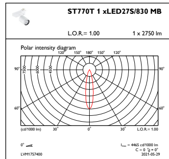
OFPC1_ST770T1xLED27S830MB
