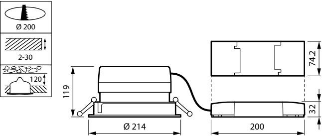
DN571B LED24S/840 PSU-E C WH
