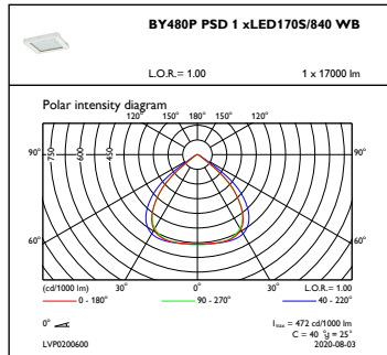
OFPC1_BY480PPSD1xLED170S840WB
