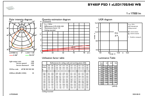
IFGU1_BY480PPSD1xLED170S840WB
