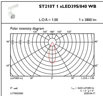
OFPC1_ST210T1xLED39S840WB
