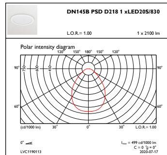
OFPC1_DN145BPSDD2181xLED20S830
