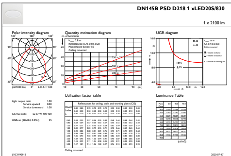
IFGU1_DN145BPSDD2181xLED20S830
