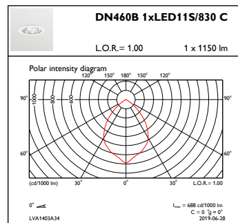
OFPC1_DN460B1xLED11S830C
