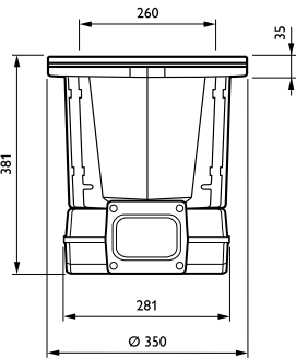
BBP623 34xLED-HB/WW II NB GC GR RMR
