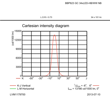
OFCC_BBP623 GC 34xLED-HB/WW NB-Cartesian Outdoor (combined)
