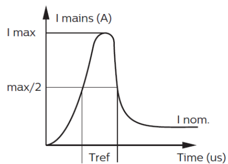
Inrush current
