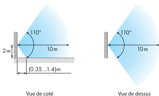
18.01, 18.11, 18.A1 - Montage mural
