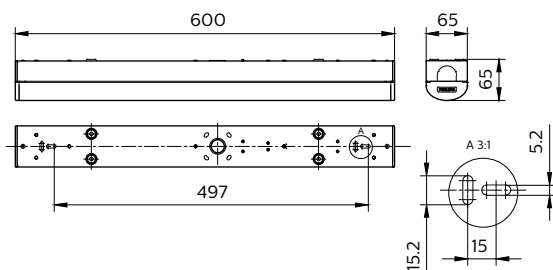
BN126C LED22S/840 PSU L600
